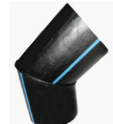
Fabricated 22.5° Elbow
